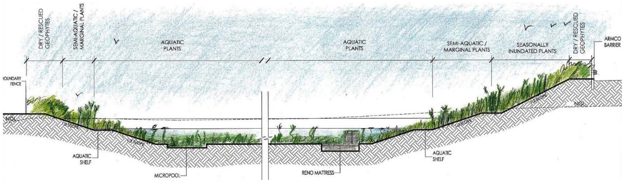
ATTENUATION POND 1: SECTION B-B
