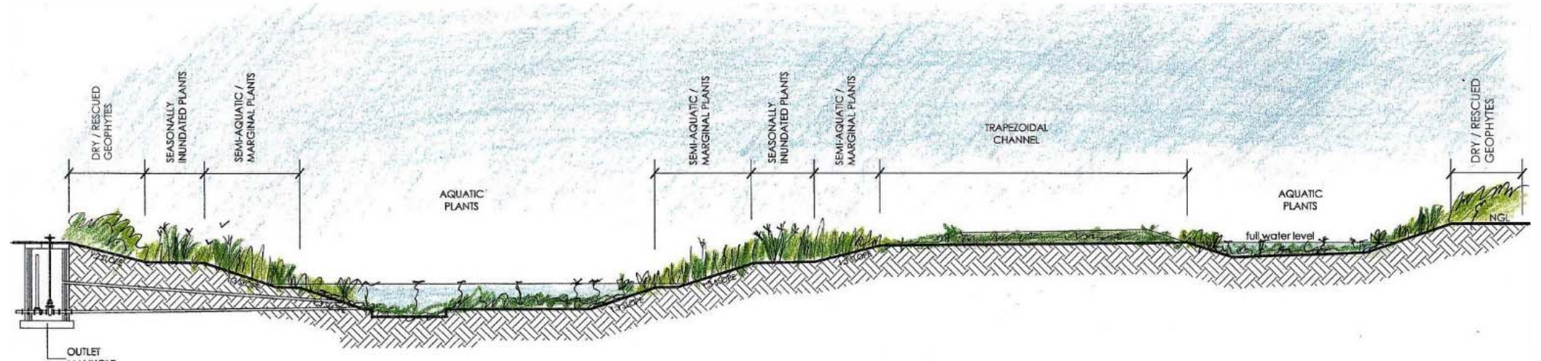
ATTENUATION POND 2: SECTION C-C
